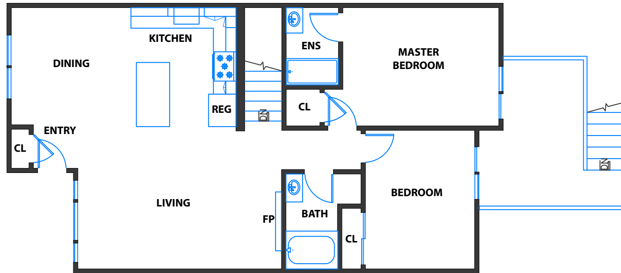
UPPER LEVEL
